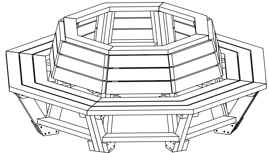
3D View of tree seat assembly
