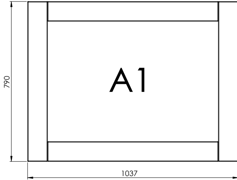
A1 Lectern Viewable Area Size - W847 x H594 Frame constructed from 100 x 40 lumber Supplied assembled with 2no. Legs Legs constructed from 100 x 100 lumber
